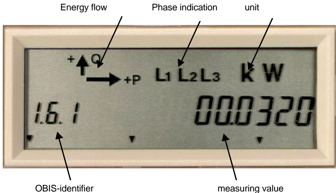
Fig. 2 LC display of the A2500 in conformity with VDEW Specification V2.0
