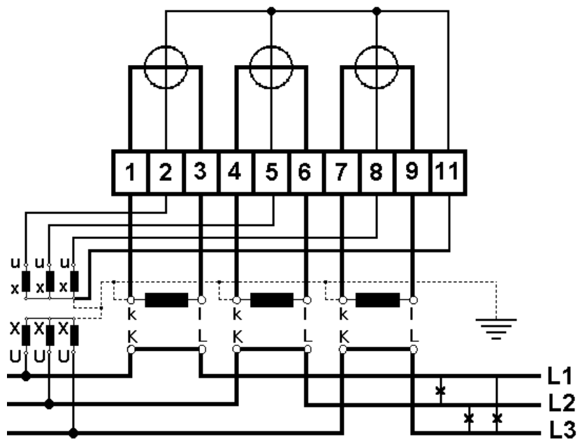
Fig. 20: 4-wire meter for CT- and VT-connection
