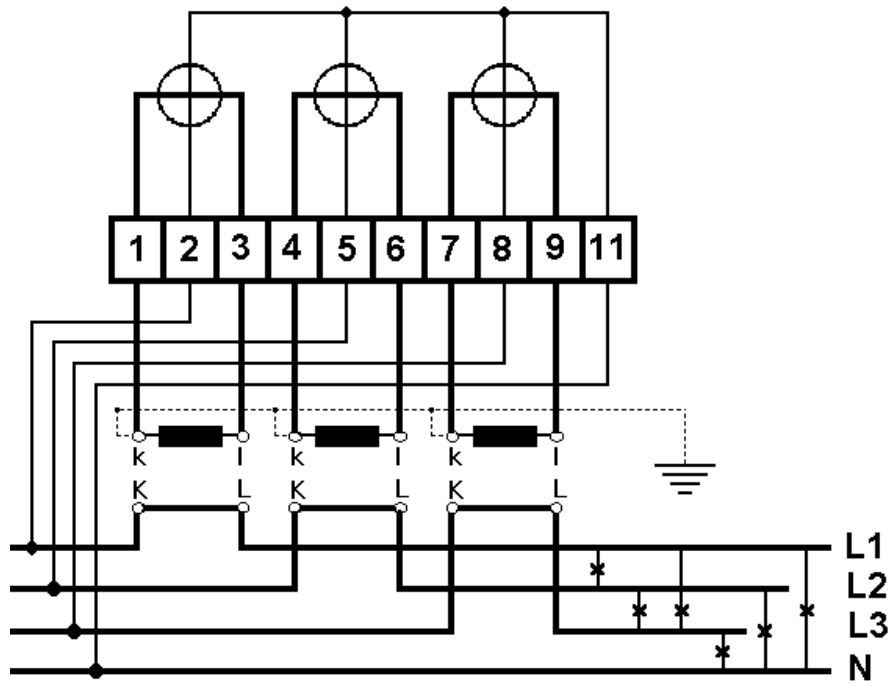
Fig. 19: 4-wire meter for CT connection
