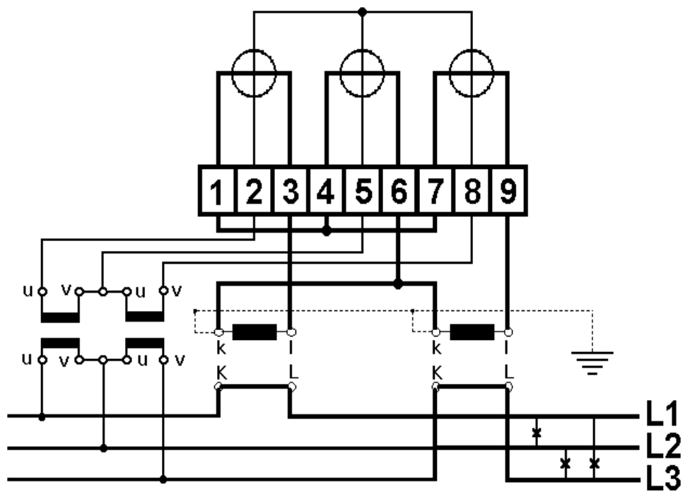
Fig. 22: 4-wire meter without connection of the neutral
