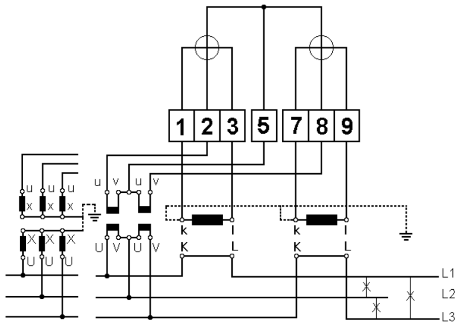
Fig.21: 3-wire meter for CT- and VT-connection
