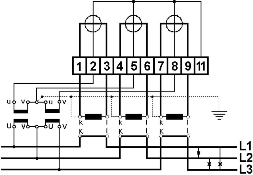
Fig. 23: 4-wire meter without connection of the neutral
