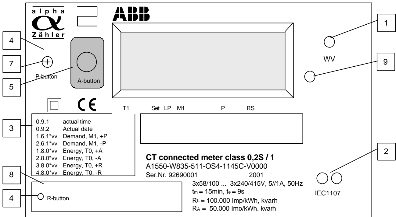
Fig 16: Front view of the meter
