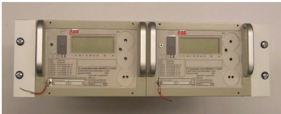
Fig. 11 A2500 installed in a 19" rack
