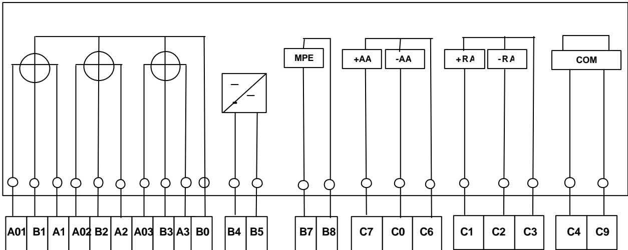
Fig. 14: Connection diagram
