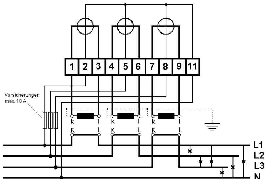
Fig.17 Connection of a CT meter in the low voltage level
