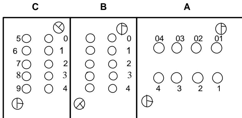
Fig. 15 Essalec connectors
